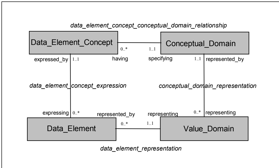
Figure 3: High-level metamodel
