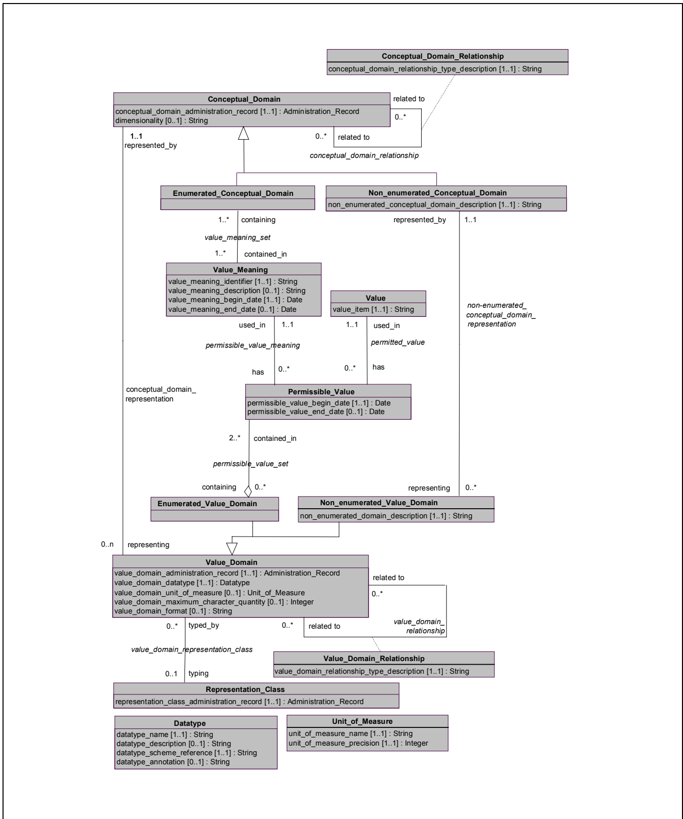
Figure 9: Conceptual and value domain metamodel region
