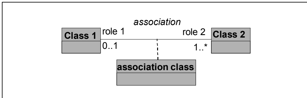
Figure B-6: Notation for "Association Class"
