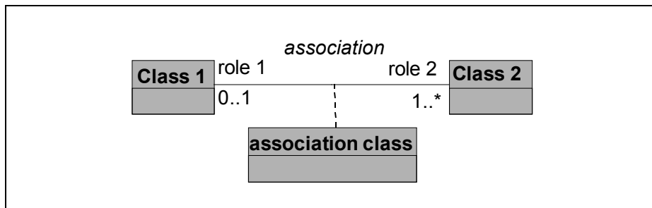
Figure B-6: Notation for "Association Class"
