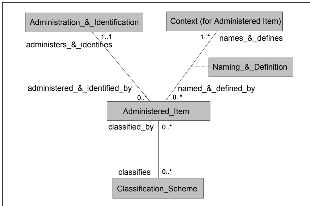
Figure 1: Common facilities for all Administered Items
