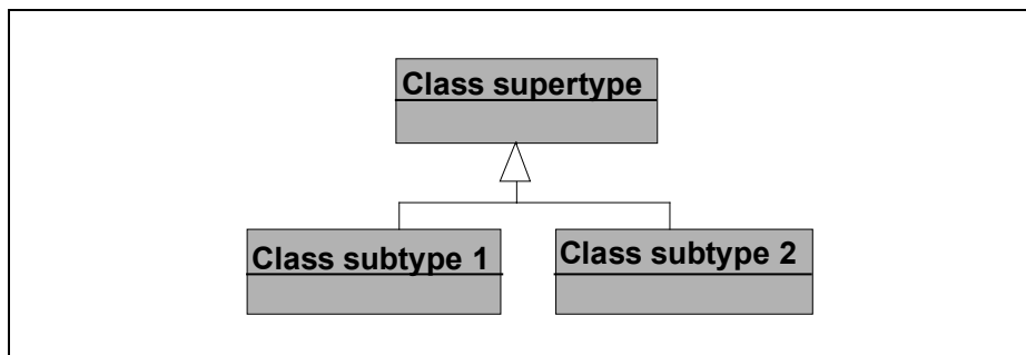
Figure B-7: Notation for Supertype / Subtypes
