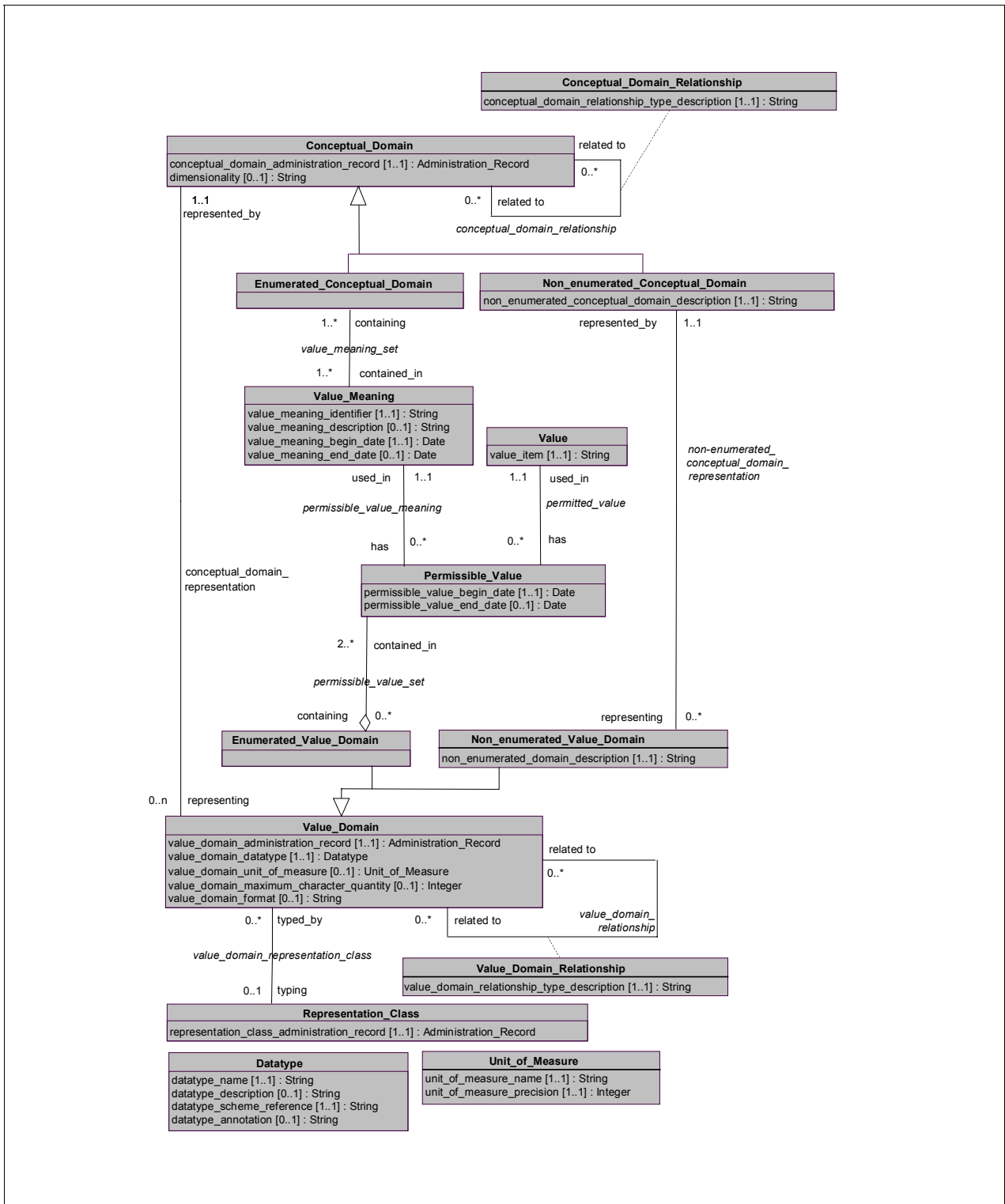
Figure 9: Conceptual and value domain metamodel region
