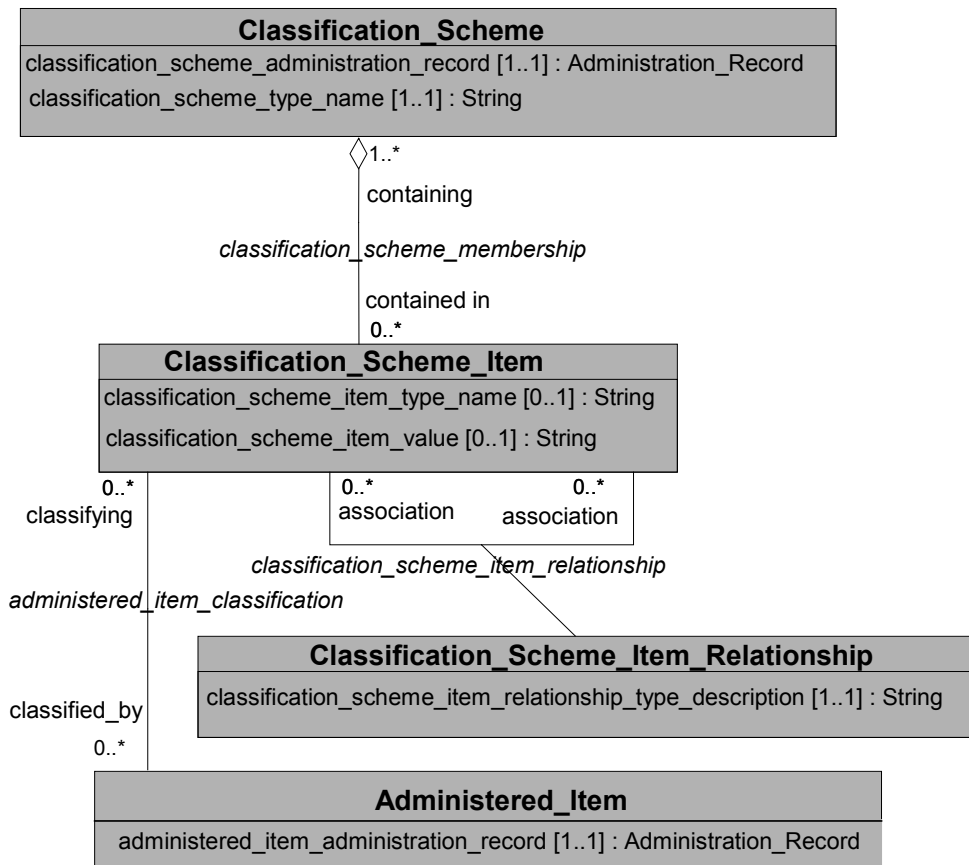
Figure 7: Classification metamodel region
