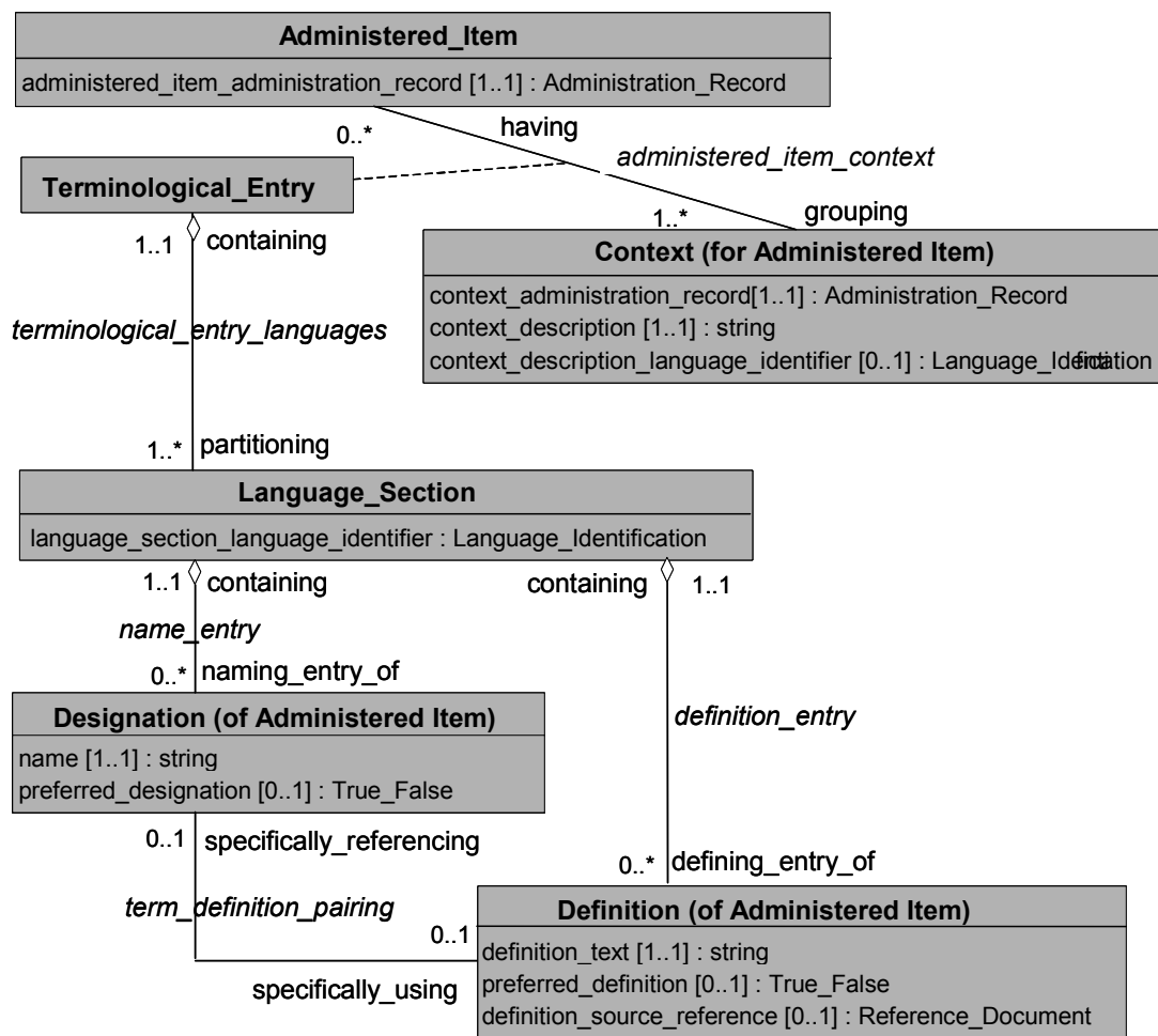
Figure 6: Naming and Definition metamodel region
